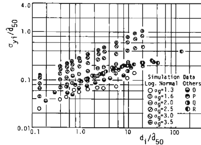
Fig. 8 Standard Deviation of Height of Exposed Particles for Each Grain Size.
