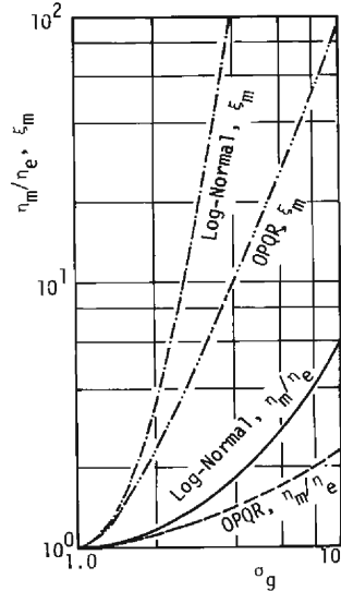
Fig. 19 \eta_m/\eta_e \epsilon_m \sigma_g \equiv \sqrt{d_{84}/d_{16}} .
