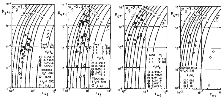
Fig. 25 Sediment Pick-up Rate for Each Grain Size of Sand Mixture.
