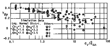
Fig. 11 Correlation Coefficient of Angle of Escape and Height of Exposed Particles for Each Grain Size.
