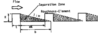
Fig. I Separated Zone of Flow in Downstream of Roughness Element.
