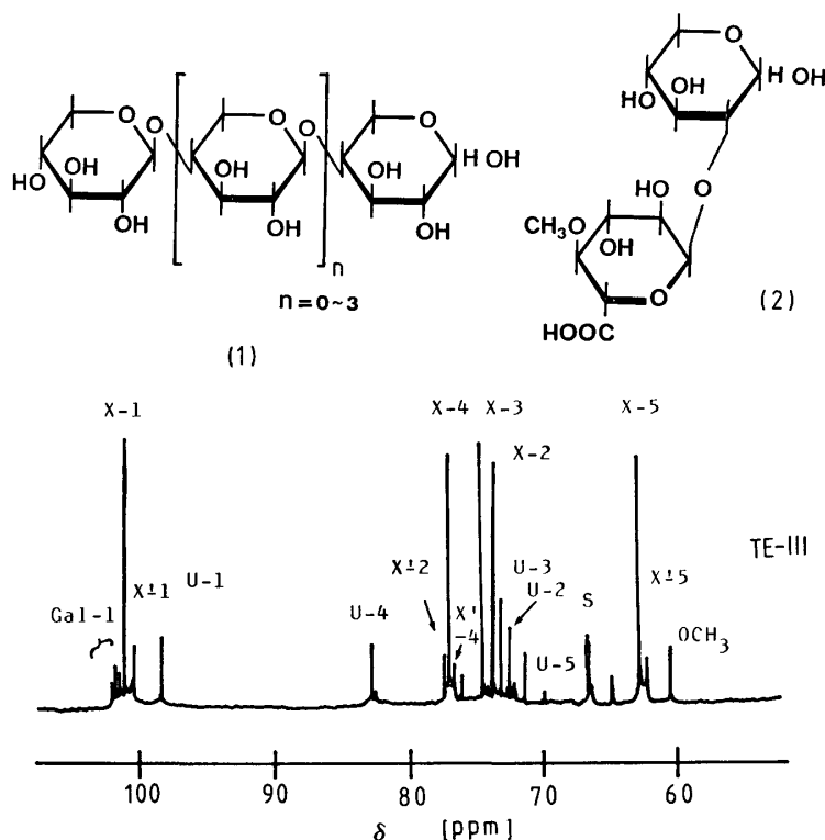
Fig. 3-(a) ^{13}\text{C} -N.m.r. spectrum of the TE-III fraction. X, U and Gal indicate xylose, 4- O -methylglucuronic acid and galactose residues, respectively. X' indicates xylose residue substituted at C-2. S indicates 1,4-dioxane as an internal standard.
