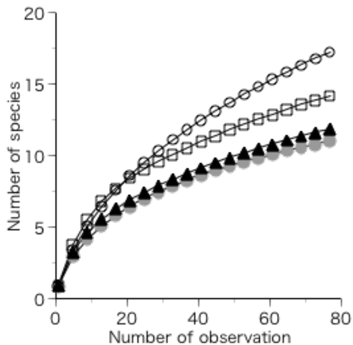
Fig. S2. Rarefaction curves for litter-decomposing macrofungal (LDM) assemblages. □, subtropical forest (ST); ○, lower part of a slope in cool temperate forest, [CT (lower)]; ●, upper part of a slope in cool temperate forest [CT (upper)]; ▲, subalpine forest (SA).
