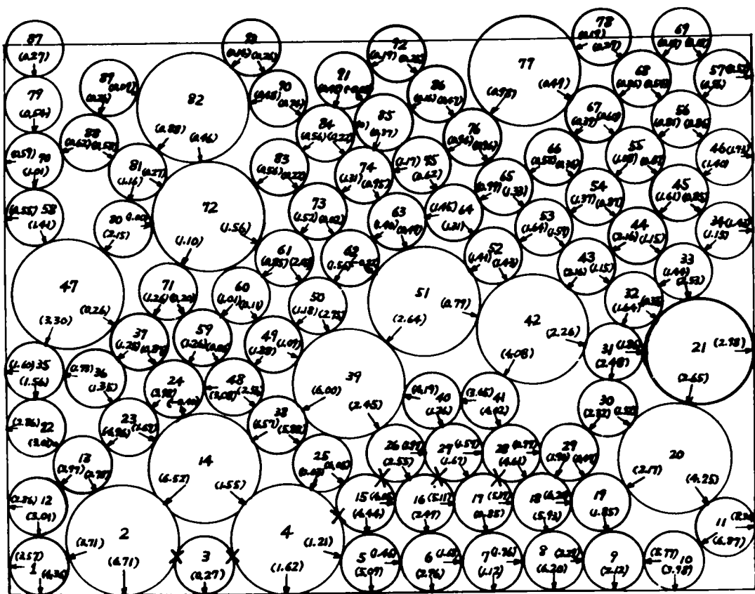
Fig.1.2.1 Simulation of two-dimensional particle arrangement obtained by applying Monte Carlo method and transmission of interparticle force due to own weight of particles (in the case of two diameters).
