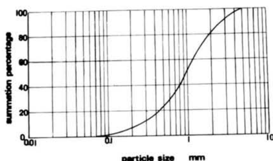
Fig.1.3.4 Grain size distribution curve of Ishii River sand.
