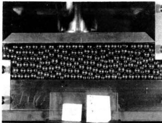
Photo.1.2.6 Particle arrangement of steel balls ( \phi 4, 6.3, 8\text{mm} ) during shear.
