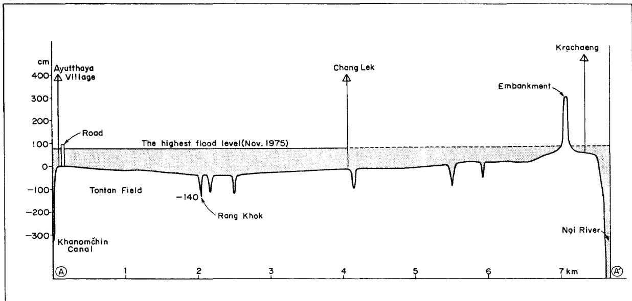
Fig. 2 Profile of the Cross Section A-A'
