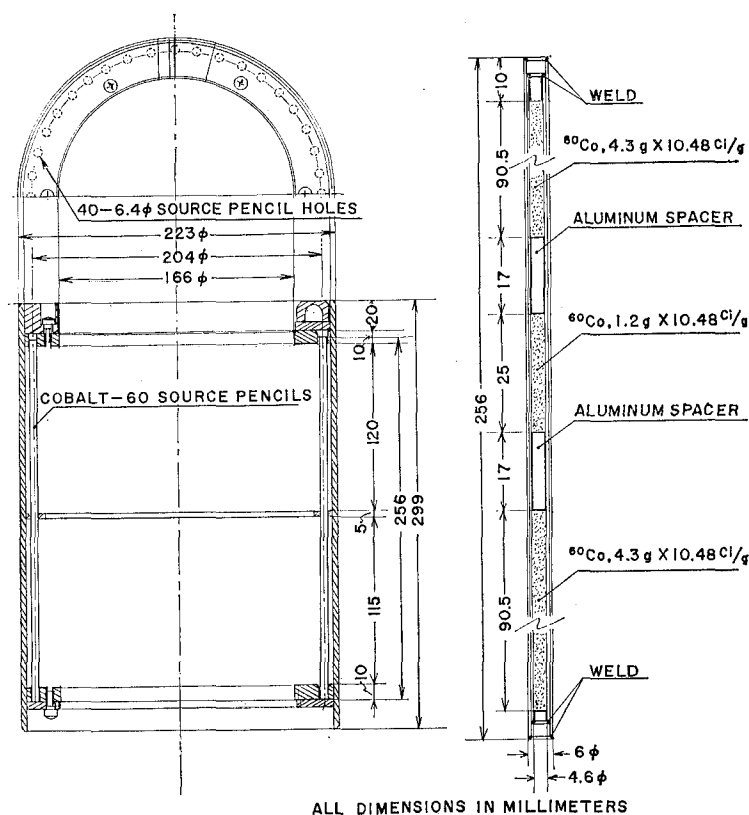
Fig. 3. Vertical and horizontal sections of the annular source cage and cross section of the 60 Co source pencil.
