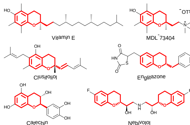
Fig. 1 Representative 2-substituted chromans in bioactive compounds.
