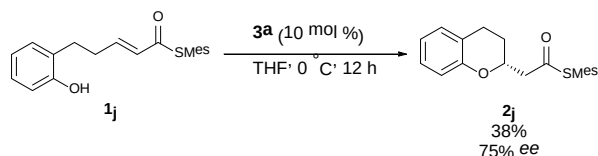
Scheme 3 Reaction of \alpha,\beta -Unsaturated Thioester
