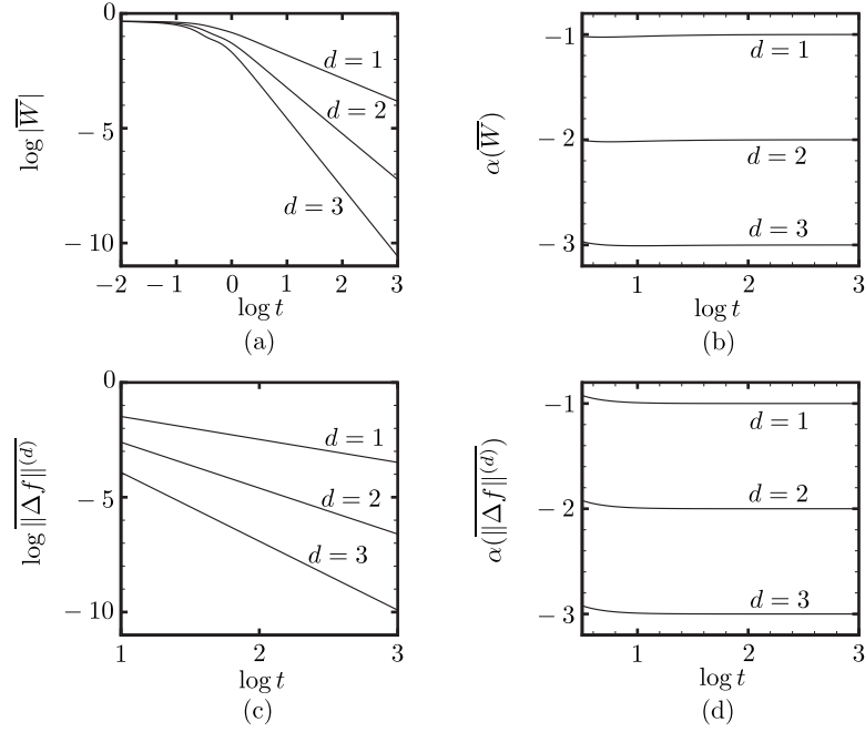
Fig. 2.7 Long-time behavior of \overline{W} and \|\Delta f\|^{(d)} for different dimension d = 1, 2 , and 3 for T_0 = 2 . (a) \log |\overline{W}| vs \log t , (b) \alpha(\overline{W}) vs \log t , (c) \log \|\Delta f\|^{(d)} vs \log t , (d) \alpha(\|\Delta f\|^{(d)}) vs \log t .
