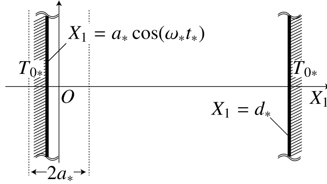
Fig. 4.1 A gas between an oscillating plate and a stationary plate.
