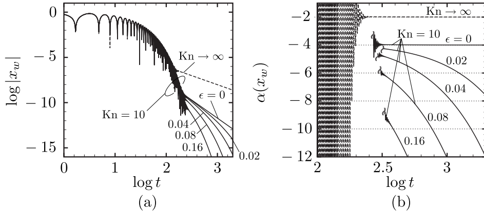
Fig. 3.8 The decay of the displacement x_w(t) for d = 1 , M = 10 , x_{w0} = 1 , and v_{w0} = 0 [special Lorentz gas with moving obstacle: Eq. (3.12)]. (a) \log_{10}|x_w| vs \log_{10} t . (b) The gradient \alpha(x_w) of the curve in panel (a) vs \log_{10} t .
