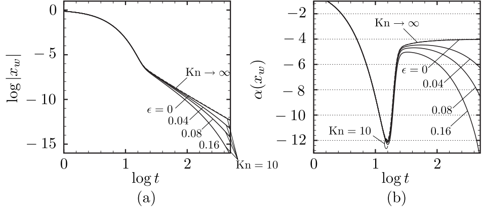
Fig. 3.9 The decay of the displacement x_w(t) for d = 3 , M = 1 , L = 1 , x_{w0} = 1 , and v_{w0} = 0 [special Lorentz gas with moving obstacle: Eq. (3.12)]. (a) \log_{10} |x_w| vs \log_{10} t . (b) The gradient \alpha(x_w) of the curve in panel (a) vs \log_{10} t .
