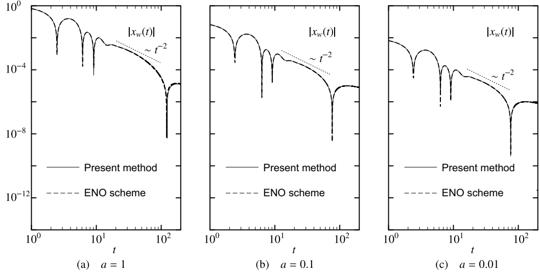
Fig. 4.22 The displacement |x_w(t)| vs t in double logarithmic scale for K = 10 . (a) a = 1 , (b) a = 0.1 , and (c) a = 0.01 . The solid line indicates the results obtained by the present method, the bold dashed line those by the ENO scheme, and the bold dot-dot-dashed line and the bold dot-dashed line in panel (a) those by the ENO scheme with coarser grid systems.
