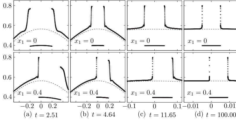
Fig. 2.5 Time evolution of the marginal velocity distribution function \tilde{f}(x_1, \zeta_1, t) for T_0 = 2 in the 1D case ( d = 1 ). (a) t = 2.51 , (b) t = 4.64 , (c) t = 11.65 , (d) t = 100.00 . Figures (a), (b), (c) and (d) are enlarged figure of Fig. 2.4 (e), (f), (g) and (h), respectively. See the caption of Fig. 2.4.
