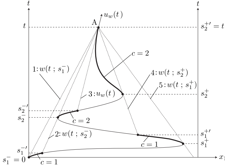
Fig. 1.4 Trajectory of the plate and definitions of the symbols.
