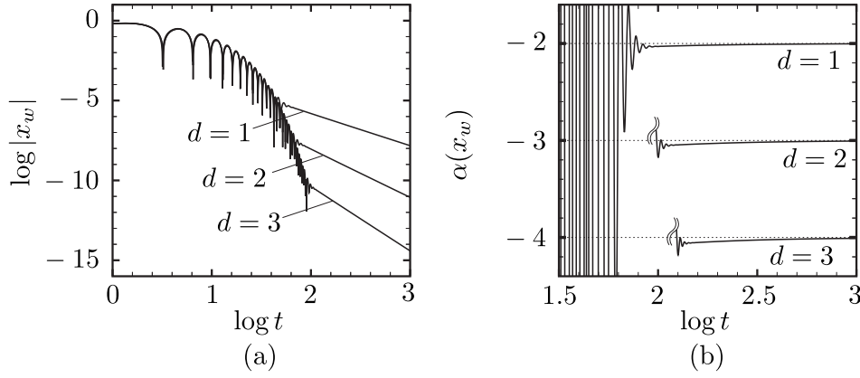
Fig. 3.4 The decay of the displacement x_w(t) for d = 1, 2 , and 3 in the case of M = 4 , L = 1 ( d = 2 and 3 ), x_{w0} = 0 , and v_{w0} = 1 (collisionless gas: \text{Kn} = \infty ). (a) \log_{10} |x_w| vs \log_{10} t . (b) The gradient \alpha(x_w) of the curve in panel (a) vs \log_{10} t .
