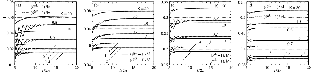
Fig. 4.12 Momentum transfer over a period \bar{\mathcal{P}}^\beta versus time ( 5 \leq t/2\pi \leq 20 ) for different M and K . (a) M = 0.1 , (b) M = 0.2 , (c) M = 0.5 , and (d) M = 1 . The solid line indicates (\bar{\mathcal{P}}^L - 1)/M , and the dashed line (\bar{\mathcal{P}}^R - 1)/M .
