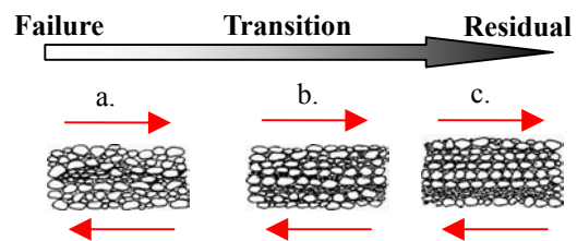
Fig. 13 The hypothetical mechanism of shear zone development process in accordance to its structural development process on granular (cohesionless) material which correspond to the shear deformation process under undrained condition by means of ring shear
