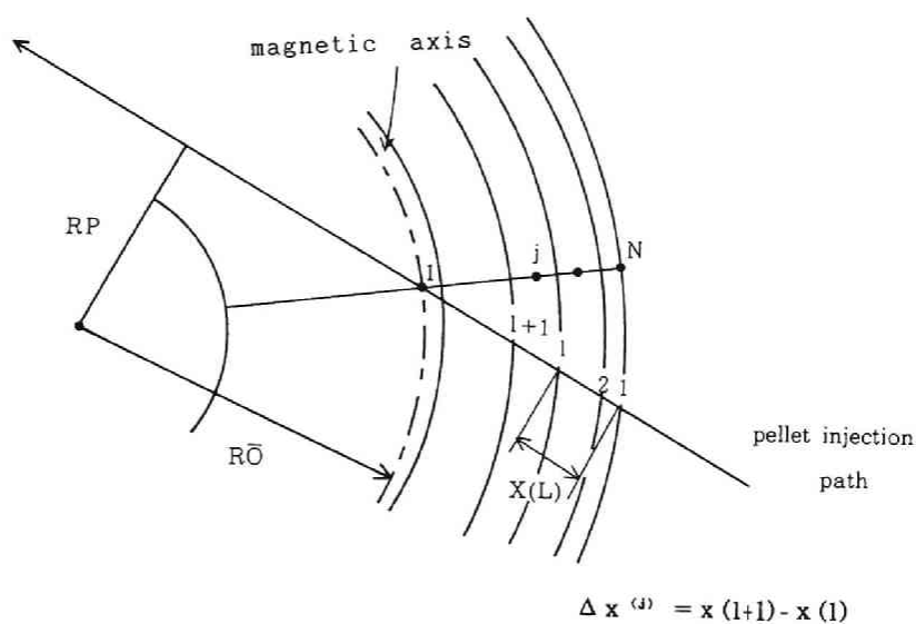
Fig.5.2. Top view of plasma column and pellet injection path.
