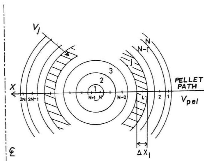
Fig.5.1. Spatial meshes of plasma column. \Delta x_l is path length of pellet through l-th mesh region (or j-th mesh region), and V_j is volume contained in j-th mesh region.
