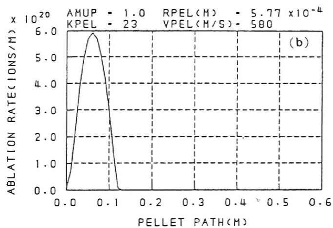
Fig.7.3. Ablation rate profiles calculated from (a) PT model and (b) Milora model for pellet injection into high-power NBI heated plasma of Heliotron E.
