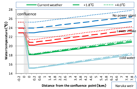
Fig. 18 Calculation result of water temperature
