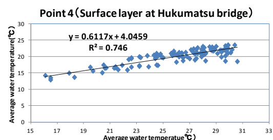
Fig. 12 Relation between air temperature and water temperature at Point 4 (2011/5/28～9/13)
