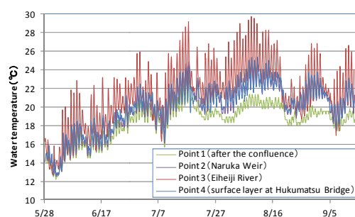
Fig. 7 Observed value of water temperature
