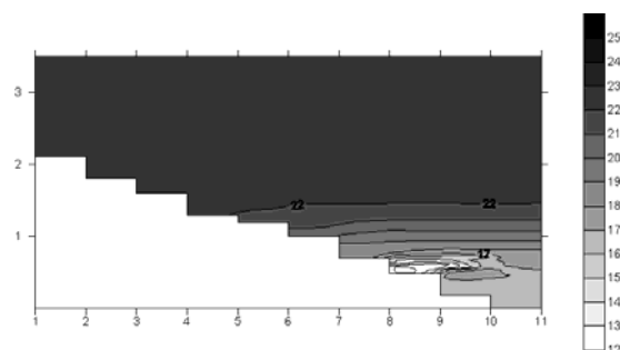
Fig. 25 Distribution of water temperature (depth:3m, spring point C)
