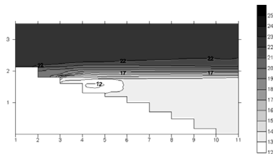
Fig. 24 Distribution of water temperature (depth:3m, spring point B)
