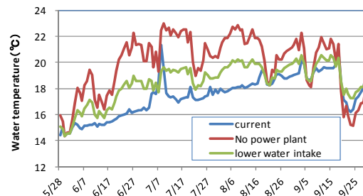
Fig. 15 Water temperature after the confluence based on intake conditions by the power plant
