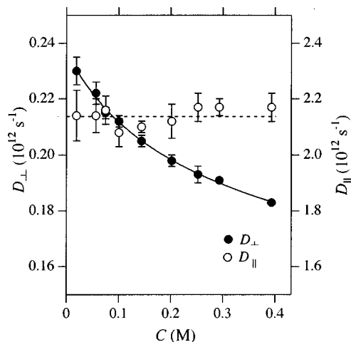
FIG. 1. Concentration dependence of the rotational diffusion coefficients of the tumbling ( D_\perp ) and the spinning ( D_\parallel ) motions of \text{CD}_3\text{CN} in \text{C}_6\text{H}_{14} at 30^\circ\text{C} .
