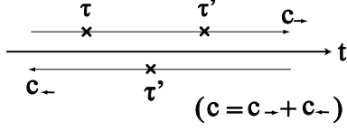
Fig. A-1. Keldysh contour, c . We have taken \tau on forward path, c_+ . Even when \tau is located on backward path, c_- , the result of this calculation is invariant because each Green's function, G^r , G^a , G^< , G^> (the greater Green's function), is not independent; they obey, G^r - G^a = G^> - G^< . Both the forward and backward paths are actually on the real axis but shifted slightly upwards and downwards, respectively, to distinguish them clearly.
