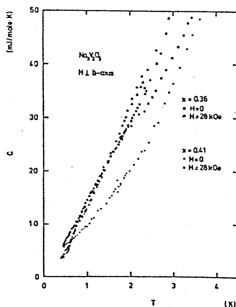
\beta\text{-Na}_x\text{V}_2\text{O}_5 の磁場中比熱 ( C - T )
