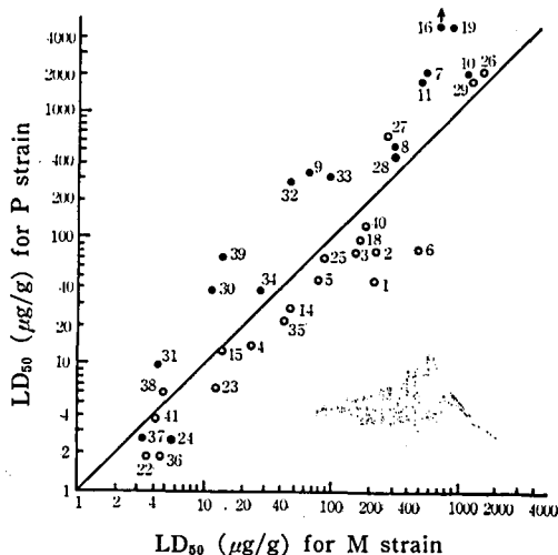
Fig. 3. Relationship between LD 50 values for M and P strains of various organophosphorus compounds.
