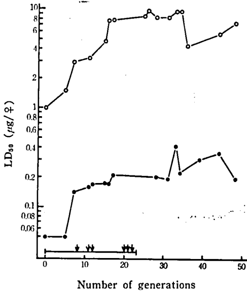
Fig. 2. Changes of LD_{50} ( \mu\text{g}/\text{female} ) of malathion and methyl parathion through generations of the population selected with methyl parathion.
