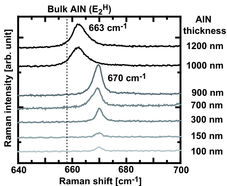
Figure 5.21: Raman spectra of AlN layers on 6H-SiC (0001). AlN layers with thickness between 100 and 1200 nm were grown with 2ML-Ga pre-deposition at 650°C.
