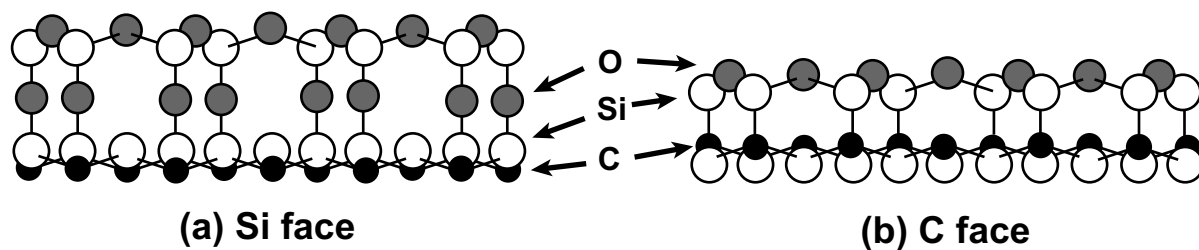
Figure 3.23: Sideview of oxide structures on (a) SiC (0001) Si and (b) SiC (000 \bar{1} ) C in [1\bar{1}00] projection.
