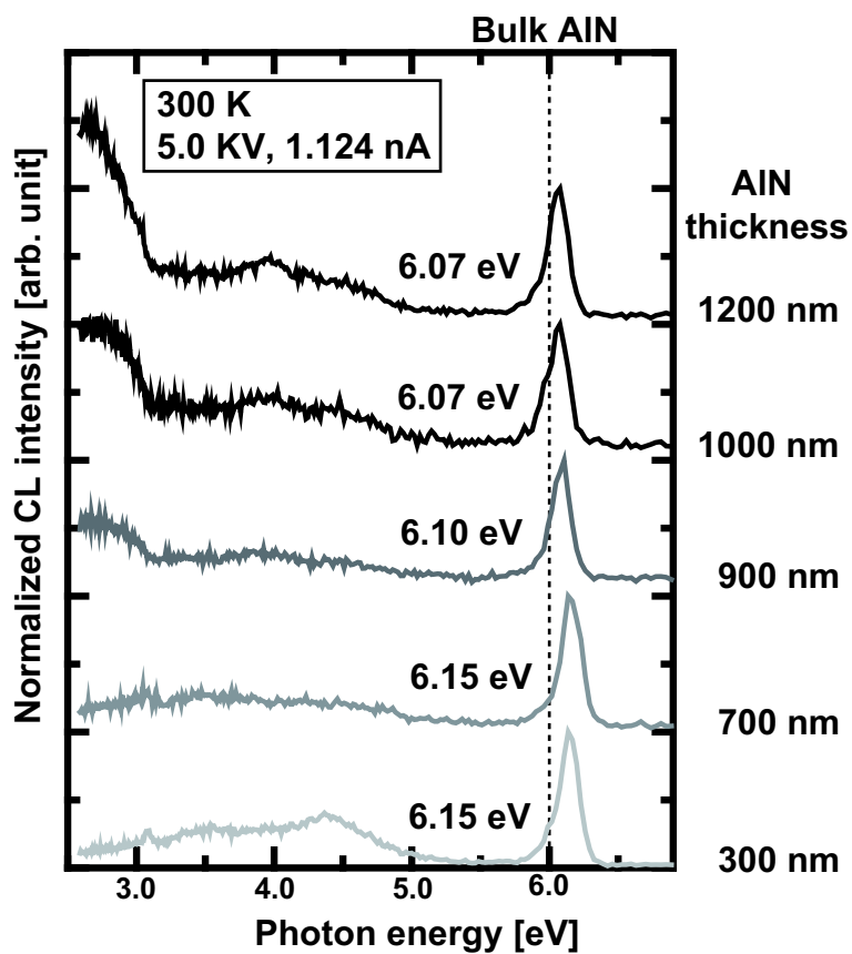
Figure 5.22: CL spectra of AlN layers on 6H-SiC (0001) at room temperature. AlN layers with thickness between 300 and 1200 nm were grown with 2ML-Ga pre-deposition at 650°C.
