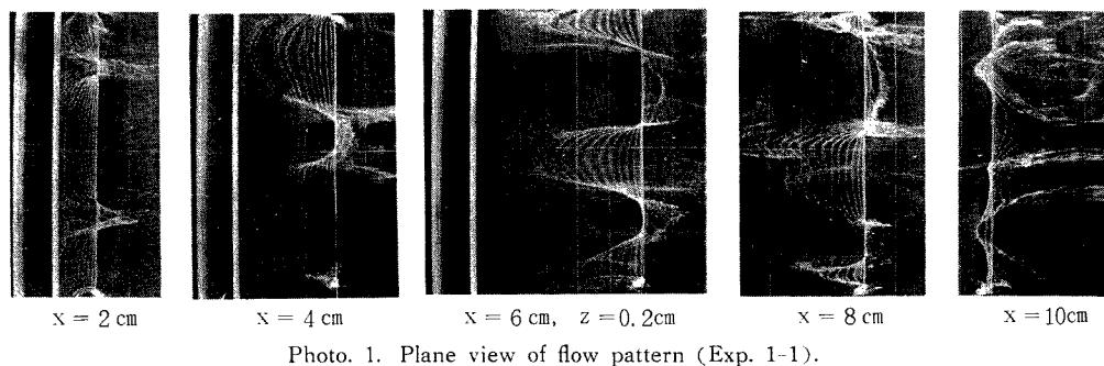
Photo. 1. Plane view of flow pattern (Exp. 1-1).
