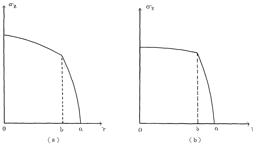
Fig. 12. The schemata of the stress distribution in the case using a ring, (a) in the ordinary case and (b) in the ideal case in which m is naught inside the ring.
