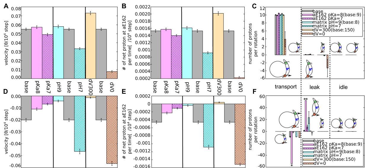
Figure 5. The effect of the parameters, pK_a , pH , \Delta\Psi on the model F_0 functions. The rotational velocities, numbers of net proton movement per time and per rotation, are plotted with no external torque in the ATP synthesis mode (A–C) and a strong torque 86.2 \text{ pN} \cdot \text{nm} in the ATP hydrolysis mode (D–F). The pK_a value does not strongly affect both the rotational velocities and the number of transferred protons in the ATP synthesis mode (A–C) but decreases that of the ATP hydrolysis mode (D–F). The pH and \Delta\Psi differences affect in the expected way. With strong proton motive force, ATP synthesis activity increases and proton pumping activity is inhibited. Note that the values indicated with “*”, “**”, and “†” mean 42.3, 42.5, and N/A, respectively.
