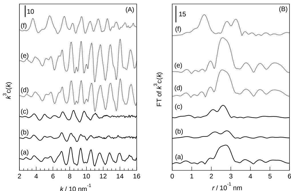
Figure 9 k^3 -weighted EXAFS oscillation at Pt L_3 -edge (A) and their Fourier transforms (B) of Pt-Sn/SiO 2 reduced at 1073 K, Pt/SiO 2 , and Pt foil: (a) 3Pt1Sn/SiO 2 , (b) 1Pt1Sn/SiO 2 , (c) 1Pt3Sn/SiO 2 , (d) Pt/SiO 2 reduced at 773 K, (e) Pt foil, (f) PtO 2 .
