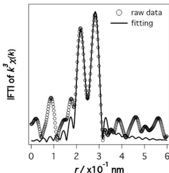
Figure 6 The curve-fitting analysis of the Pt L III -edge EXAFS data for Pt-Sn/SiO 2 ( DR ) catalyst.
