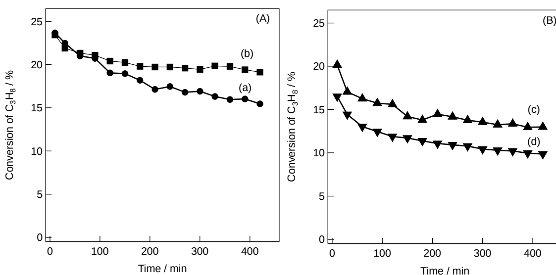
Figure 1 Time-course of propane dehydrogenation over Pt-Sn/SiO 2 catalyst. (A) 1st run, (B) 2nd run (after regeneration): (a) reduced at 1073 K, without H 2 , (b) reduced at 1073 K, with H 2 , (c) Pt-Sn/SiO 2 (R), (d) Pt-Sn/SiO 2 (OR), Reaction conditions: catalyst weight, 50 mg; reaction temperature, 773 K; (a), (c), (d) P(\text{C}_3\text{H}_8) = 20.3 \text{ kPa} ; P(\text{N}_2) = 81.0 \text{ kPa} ; (b) P(\text{C}_3\text{H}_8) = 20.3 \text{ kPa} ; P(\text{H}_2) = 5.0 \text{ kPa} ; P(\text{N}_2) = 76.0 \text{ kPa} .
