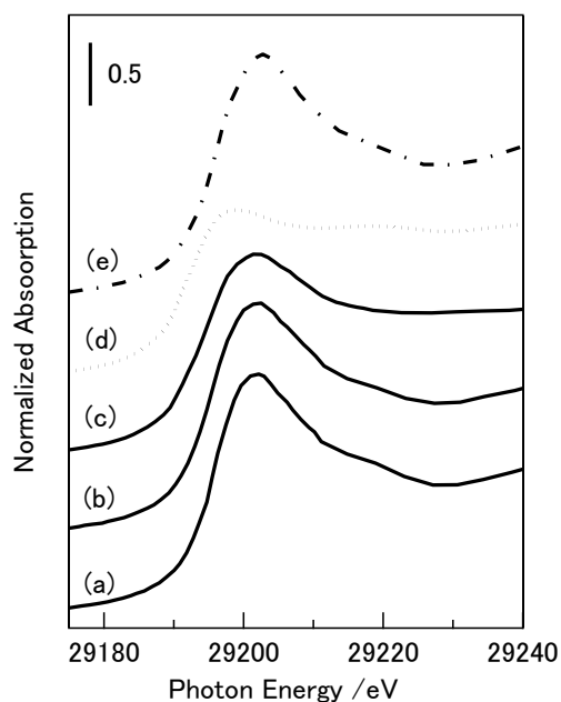
Figure 6 Sn K-edge XANES spectra of Pt-Sn/SiO 2 and references: (a) Pt-Sn/SiO 2 _1073K O 2 , (b) Pt-Sn/SiO 2 _1073K N 2 , (c) Pt-Sn/SiO 2 _1073K H 2 , (d) Sn foil, (e) SnO 2 .
