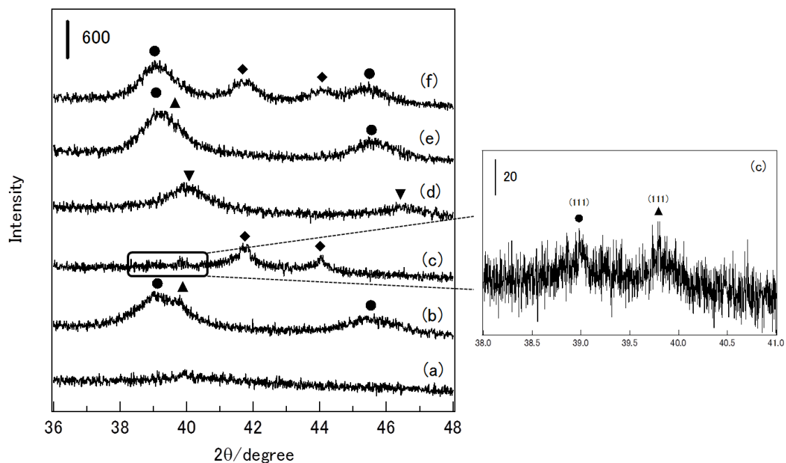
Figure 4 XRD patterns of supported Pt and Pt-Sn catalysts: (a) Pt/SBA-15, (b) 3Pt1Sn/SBA-15, (c) 1Pt1Sn/SBA-15, (d) Pt/SiO 2 , (e) 3Pt1Sn/SiO 2 , (f) 1Pt1Sn/SiO 2 . ▼: Pt metal ▲: Pt x Sn y (x/y>3) ●: Pt 3 Sn alloy ◆: PtSn alloy
