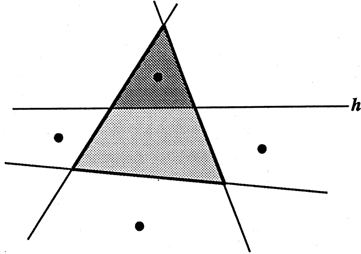
Figure 2.1. An example of \mathcal{A}(H) for 2-dimensional case. The dots show the points of T and the bold lines show the faces counted in \mathcal{A}(H - h) but not counted in \mathcal{A}(H)|T .
