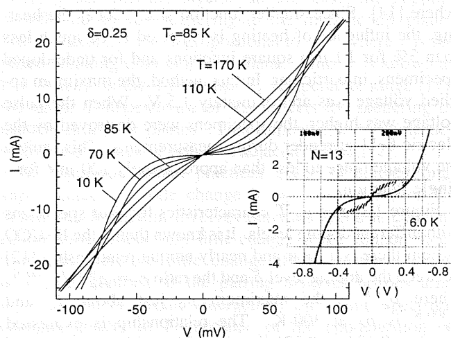
FIG. 2. I - V characteristics at different temperatures for the specimen in Fig. 1(c). The inset displays the oscilloscope I - V characteristics measured at 6 K, in which the lower branch is used for the tunneling spectroscopy.
