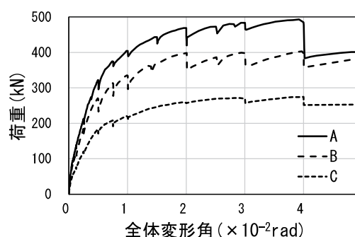
Figure 3. The skeleton curve of each
