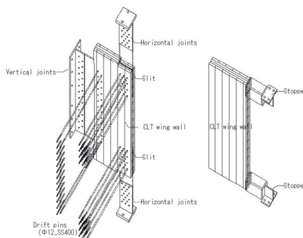
Figure 2. The specification of joint
