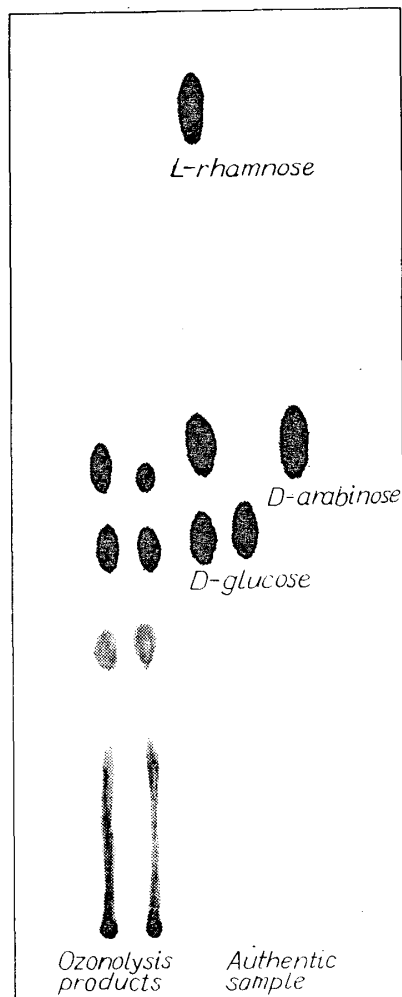
Fig. 4 PPC of ozonolysis product of haplormosin
