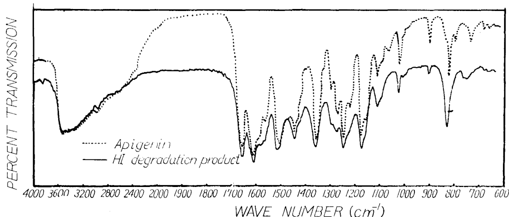
Fig. 3 IR spectra of HI degradation product of haplormosin and apigenin
