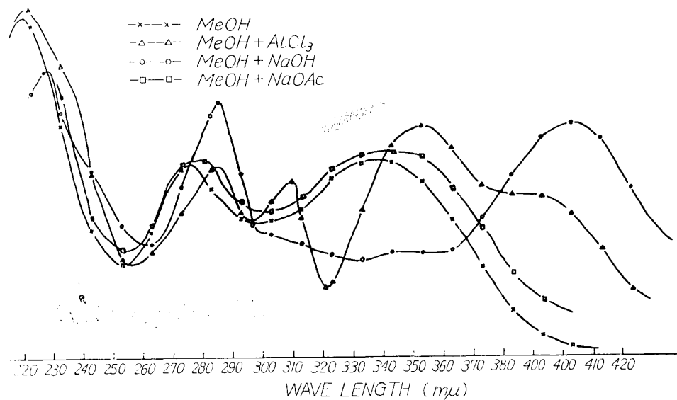
Fig. 1 UV spectra of haplormosin
