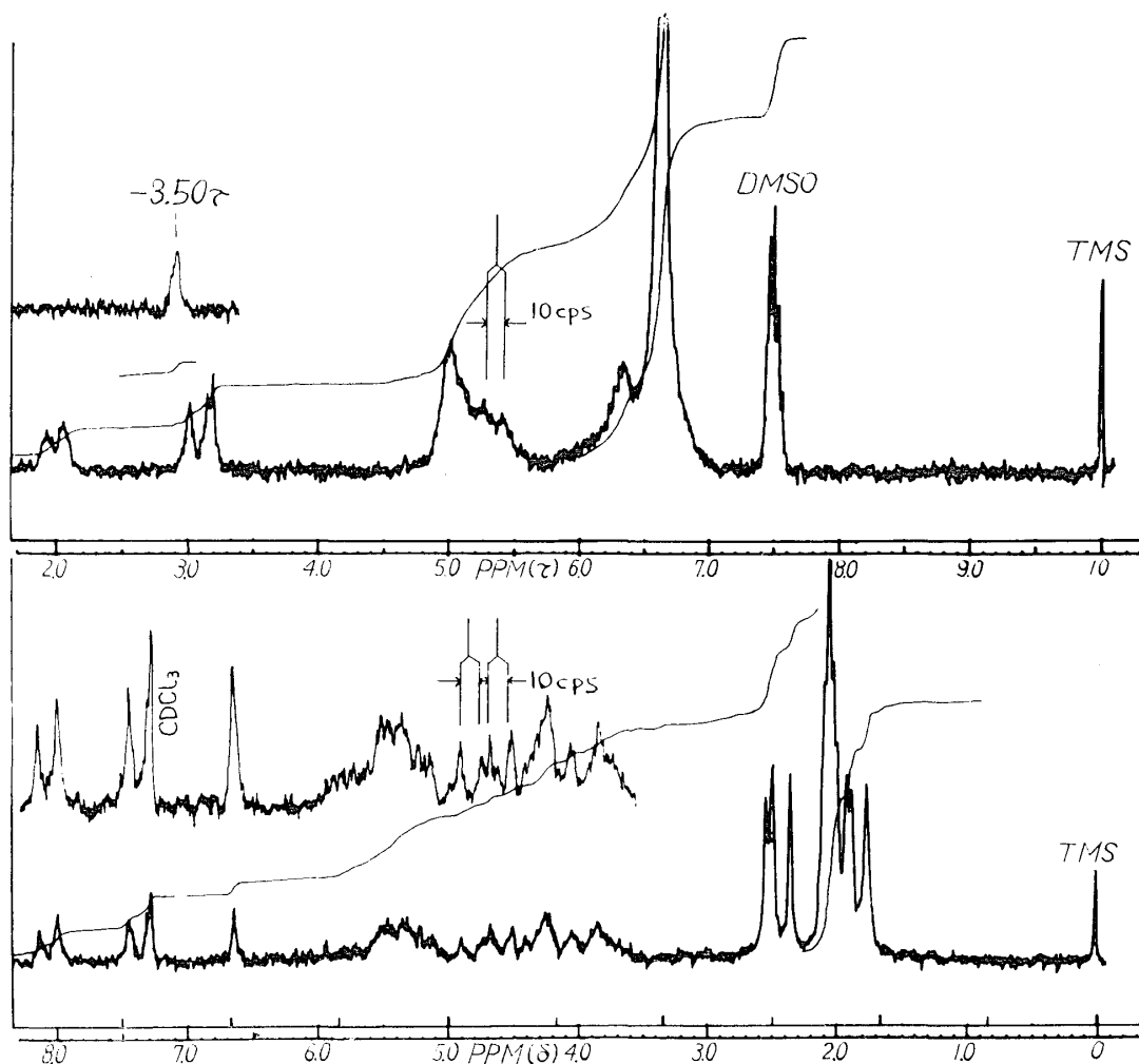
Fig. 5 NMR spectra of haploromsin and its acetate
