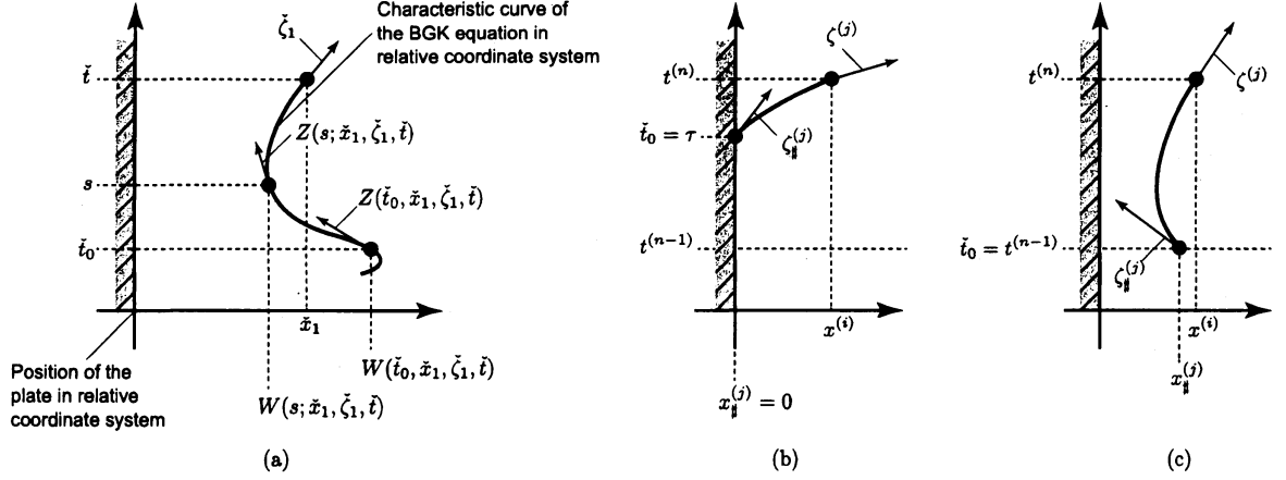
Fig. 2: Some expository figures in (\tilde{x}_1, \tilde{t}) plane, in which the gradient of the curve indicates the velocity. Therefore, a slope of arrow in the figure indicates the molecular velocity at the origin of the arrow. In the figure, we consider only the right half space \tilde{x}_1 > 0 . (a) Illustrative figure of the characteristic form (19). For a given set of (\tilde{x}_1, \tilde{\zeta}_1, \tilde{t}) , Eq. (19b) is the trajectory of a molecule in the relative coordinate system using s as a parameter. (b) Case 2 in Sec. 4.2. The characteristic curve for a given set of (\tilde{x}_1, \tilde{\zeta}_1, \tilde{t}) hits the plate at time \tau \in [t^{(n-1)}, t^{(n)}] . (c) Case 3 in Sec. 4.2. The characteristic curve for a given set of (\tilde{x}_1, \tilde{\zeta}_1, \tilde{t}) reaches a point in the gas domain without hitting the plate during the time interval [t^{(n-1)}, t^{(n)}] .
