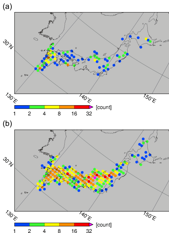
Fig. 4. The spatial distribution of the number of detection of (a) QSCCs and (b) PCCs evaluated over 50 \text{ km} by 50 \text{ km} areas for the 2017 heavy rainfall case.
