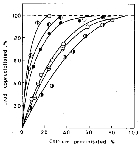
Fig. 6. The effect of pH.
