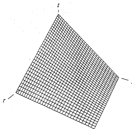
F_K: r < 1, s < 1, t < (1-r)(1-s)
