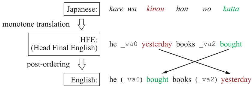
Figure 4.1: Post-ordering framework.
