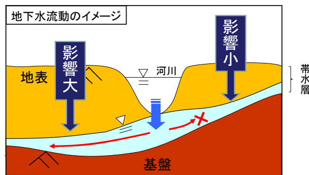
Fig. 5 Influence range of river cultivation caused by aquifer slope
