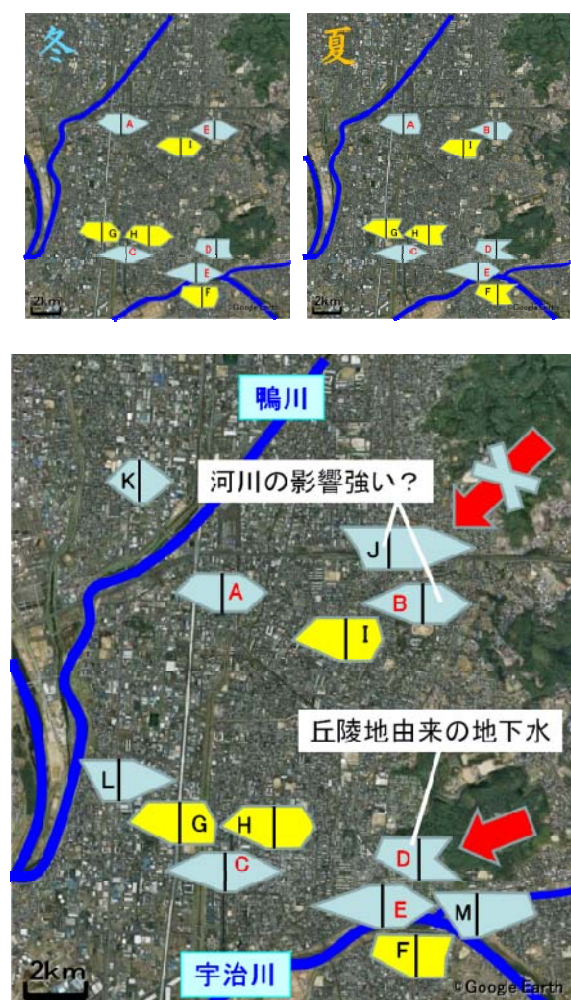
Fig. 4 Result of Hexa-diagram analysis (left-upper : average of winter season, right-upper : average of summer season, under : average of whole period)
