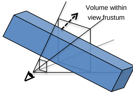
Fig. 6. The volume within the range of view frustum
