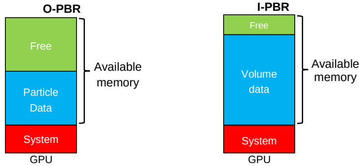
Fig. 7. Available GPU memory in O-PBR and I-PBR process.
