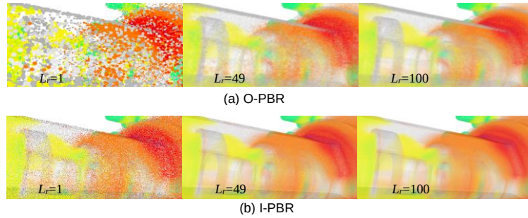
Fig. 2. Comparison of the image quality of the pump data in an enlarged view obtained by using O-PBR (a) and I-PBR (b). (Lr: repetition level)
