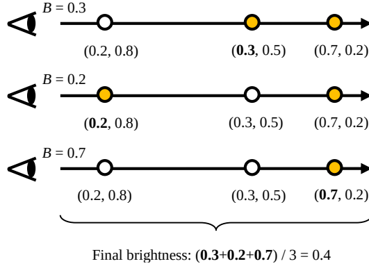
Fig. 5. Expected value of brightness.
