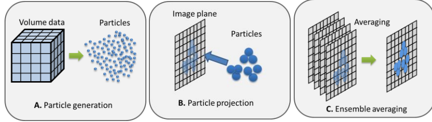
Fig. 1. The three steps of PBVR: particle generation, particle projection, ensemble average.
