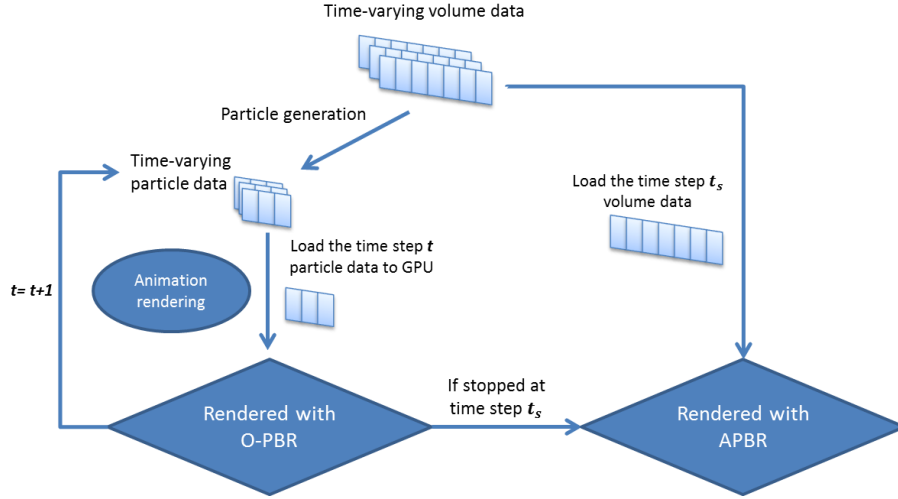
Fig. 9. The rendering process for the time-varying data.
