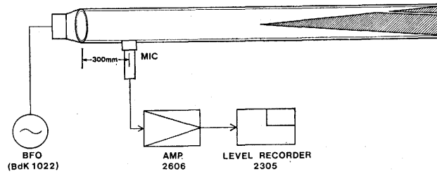
Figure 3: Measurement of the transmission characteristic of the tube.
