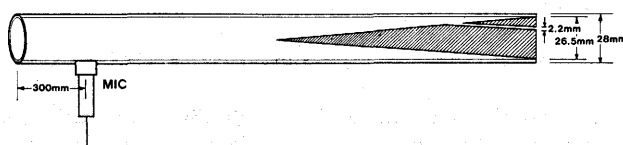
Figure 2: The reflectionless acoustic tube.
