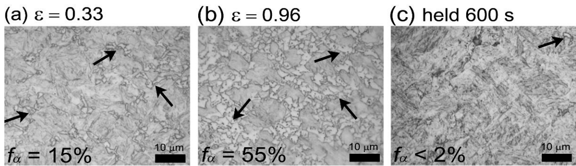
Fig. 2.3.6 Optical microscope images of the austenitized specimens deformed at 750 °C at a strain rate of 10^{-1} \text{ s}^{-1} to different strains. (a) \varepsilon = 0.33 and (b) \varepsilon = 0.96 . (c) The austenitized specimen deformed at 750 °C to a strain of 0.96, and subsequently held at the same temperature (750 °C) for 600 s after the deformation. Arrows indicate ferrite grains. Compression direction is parallel to the vertical axis in the images.
