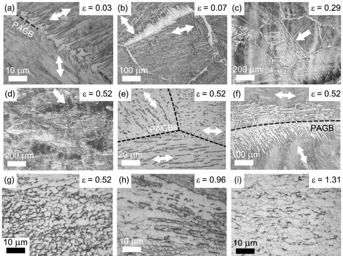
Fig. 4.2.3 Optical microscope images of specimens deformed to various strains: (a) \varepsilon = 0.03 , (b) \varepsilon = 0.07 , (c) \varepsilon = 0.29 , (d-g) \varepsilon = 0.52 , (h) \varepsilon = 0.96 and (i) \varepsilon = 1.31 . Dashed lines in (a,e,f) indicate prior austenite grain boundaries. Double-headed arrows in (a,b,e,f) represent the directions along which ferrite grains seem to be elongated. Compression direction is parallel to the vertical axis of images.
