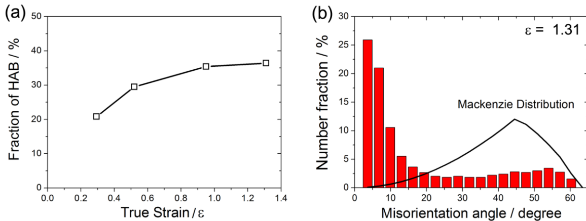
Fig. 4.2.7 (a) The change in the fraction of high angle boundaries as a function of strain. (b) The distribution of grain boundaries of the specimen deformed to a strain of 1.31 as a function of misorientation angle. Random distribution of misorientation which is known as Mackenzie distribution is plotted together [9,10].
