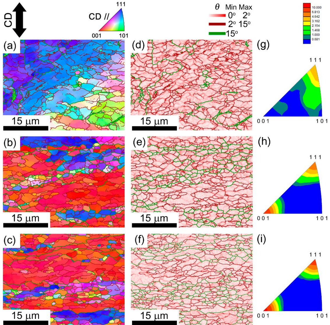
Fig. 4.2.6 (a-c) Inverse pole figure maps, (d-f) corresponding kernel average misorientation maps and (g-i) inverse pole figures of the specimens deformed to various strains: (a,d,g) \varepsilon = 0.52 , (b,e,h) \varepsilon = 0.96 and (c,f,i) \varepsilon = 1.31 . (a-f) The low angle boundaries with misorientation of 2 to 15 ° and the high angle boundaries with misorientation above 15 ° are also drawn in red and green lines, respectively. (d-f) The range of misorientation angle for kernel average misorientation is 0 to 2 °.
