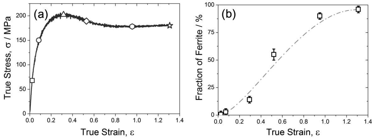
Fig. 3.3.4 (a) Stress-strain curve of the specimen deformed at a strain rate of 10^{-2} \text{ s}^{-1} to different strains at 600 °C (series 2 in Table 3.3.1). Square, circle, triangle, diamond, hexagon and star symbols indicate strains of 0.02, 0.08, 0.31, 0.5, 0.96 and 1.31, respectively. (b) Change in ferrite fraction as a function of strain.
