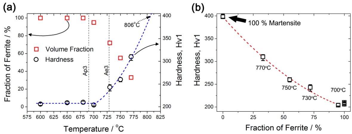
Fig. 2.3.5 (a) Changes in the fraction of ferrite and the Vickers hardness as a function of deformation temperature. Ae_3 (728 °C) and Ap_3 (684 °C) of the present material are indicated. The increase in hardness values meets the hardness of 100% martensite (398 Hv) at temperature of 806 °C. (b) Comparison between the fraction of ferrite and the Vickers hardness.
