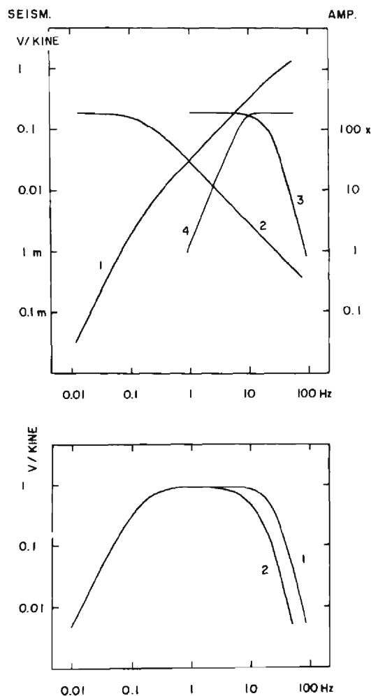
Fig. 6 Frequency characteristics of the elements of the SMS and system response. Upper: 1-seismometer (5 mV/gal, h=12 ) figured in velocity scale, 2-preamplifier with integral characteristics ( \tau=6.28 sec), 3-anti alias filter, 4-high pass filter for trigger and sample rate logic. Lower: overall responses in velocity scale, 1-100 Hz sampling, 2-50 Hz sampling with digital low pass operation.
