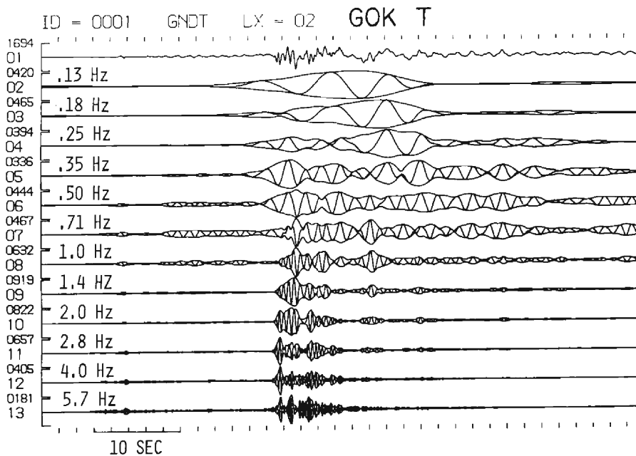
Fig. 19 (Continued) Band-pass-filtered seismograms. Maximum amplitudes are shown above trace numbers in m kine. Trace 1 is particle velocity of 0.1–10 Hz.
