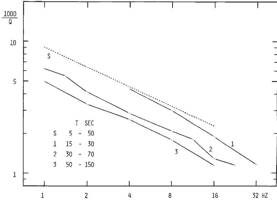
Fig. 9 Q_c^{-1} in various lapse time intervals and Q_s^{-1} for the Kinki district.
