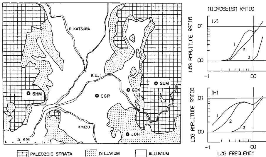
Fig. 17 Rough geological map of the southern parts of the Kyoto basin and the location of observational points. Amplification factors due to the soil deposits inferred from microseism are shown, 1: OGR/SUM, 2: GOK/SUM and 3: JOH/SUM, respectively.
