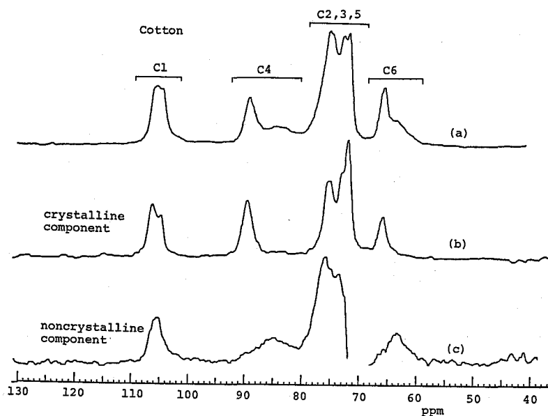
Fig. 5. 50 MHz CP/MAS ^{13}\text{C} NMR spectra of cotton. (a) whole spectrum; (b) crystalline component; (c) noncrystalline component.
