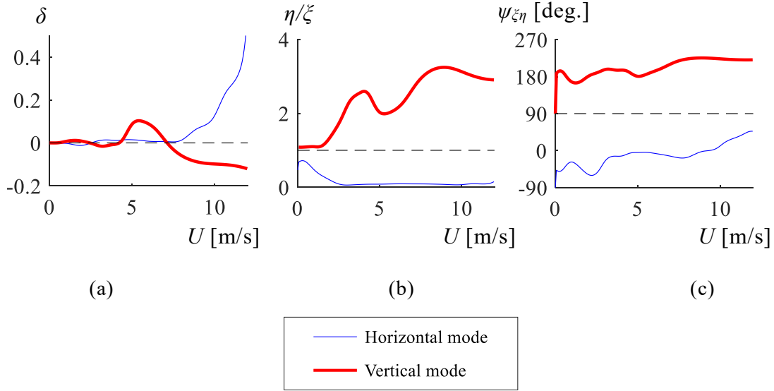
Fig. 18 Results of the flutter analysis at ( W/D = 3.0 ; S/D = 0.3 ). (a) \delta , (b) \eta/\xi , and (c) \psi_{\xi\eta} [deg.]
