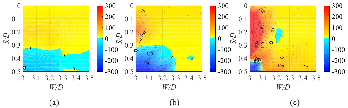
Fig. 17 Contour diagrams of H_1^* ( 2A_\eta/D = 0.4 ) (o, equilibrium position of the downstream cylinder): (a) U = 3 m/s ( U/fD = 40.5 ), (b) U = 6 m/s ( U/fD = 90.9 ), and (c) U = 12 m/s
