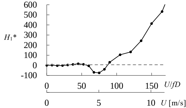
Fig. 20 H_1^* obtained from the forced vibration tests at ( W/D = 3.0 ; S/D = 0.3 ; 2A_{\eta}/D = 0.4 )
