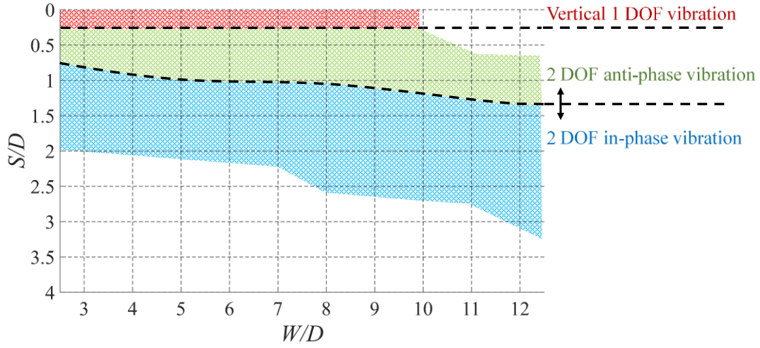
Fig. 4 Classification of the trajectories of the downstream cylinder in the spring-supported free vibration tests at U = 12 m/s
