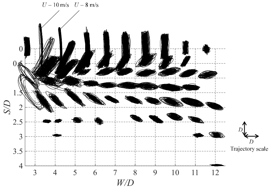
Fig. 3 Trajectories of the downstream cylinder at U = 12 \text{ m/s}
