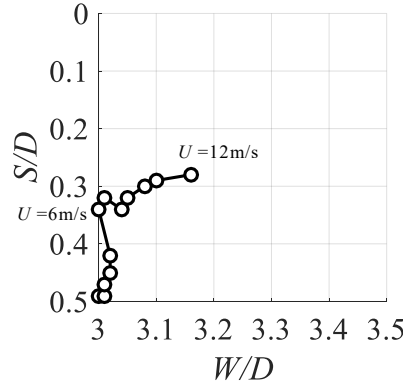
Fig. 16 Equilibrium position (static displacement) of the downstream cylinder at ( X/D = 3.0 ; Y/D = 0.5 )
