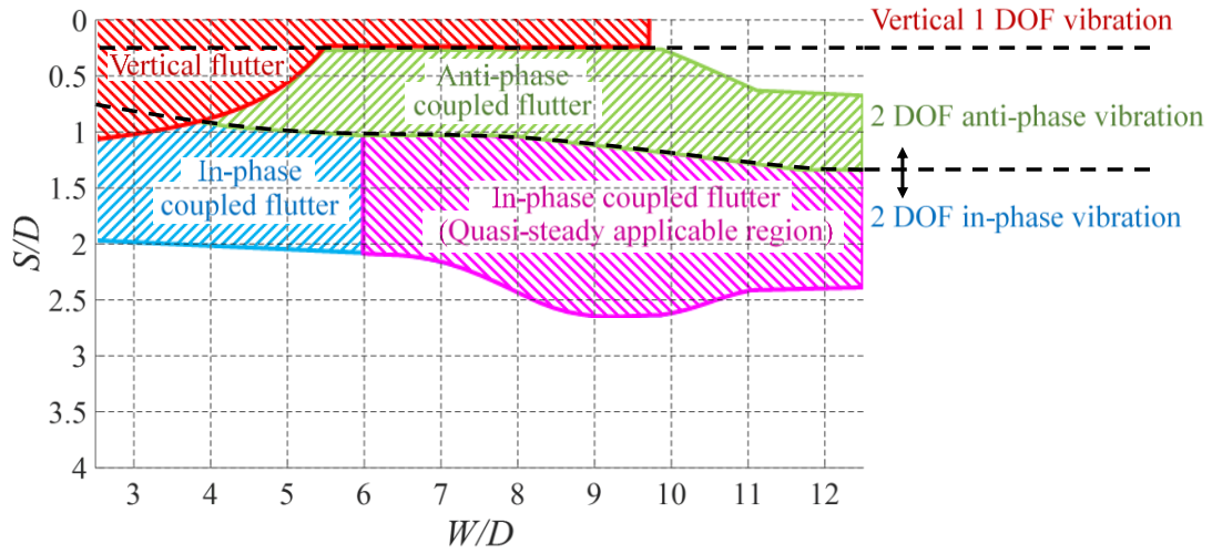
Fig. 14 Classification map of WIVs at U = 12 m/s ( U/fD = 177.8 ): Vertical flutter, vertical flutter caused by H_1^* > 0 ; anti-phase coupled flutter, 2DOF anti-phase coupled flutter caused by H_6^* < 0 , P_4^* > 0 of a short evaluation period; in-phase coupled flutter, 2DOF in-phase coupled flutter caused by the original unsteady aerodynamic derivatives or H_5^* > 0 , P_4^* > 0 of a short evaluation period
