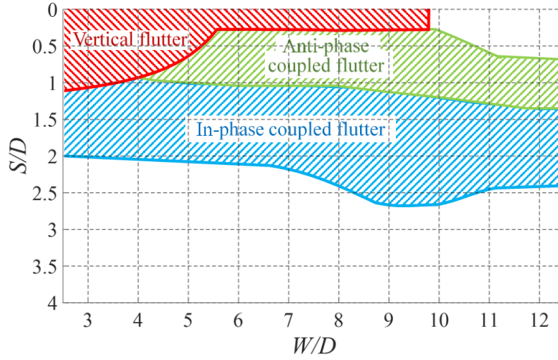
Fig. 10 Classification of vibration mechanisms based on flutter analyses at U = 12 m/s ( U/fD = 177.8 ): Vertical flutter, vertical flutter caused by H_1^* > 0 ; anti-phase coupled flutter, 2DOF anti-phase coupled flutter caused by H_6^* < 0 , P_4^* > 0 of the short evaluation period; in-phase coupled flutter, 2DOF in-phase coupled flutter caused by the original unsteady aerodynamic derivatives or H_5^* > 0 , P_4^* > 0 of the short evaluation period
