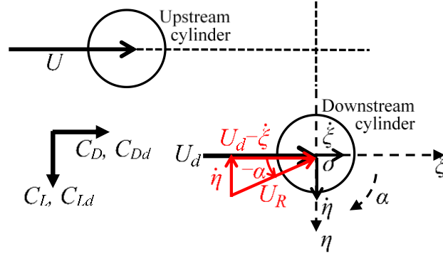
Fig. 11 Velocities and forces from the quasi-steady model
