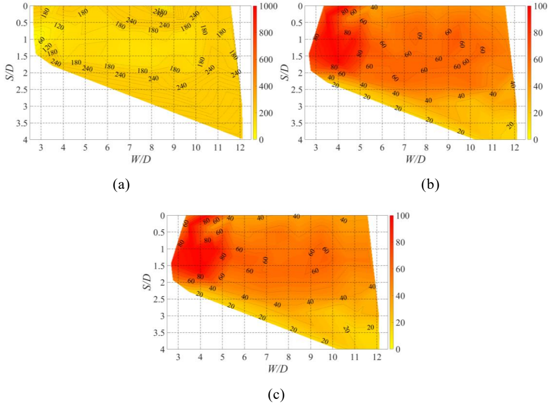
Fig. 8 Standard deviations of flutter derivatives at U = 12 m/s ( U/fD = 177.8 ): (a) P_4^* ( 2A_{\eta}/D = 0.2 ), (b) H_5^* ( 2A_{\xi}/D = 0.8 ), and (c) H_6^* ( 2A_{\xi}/D = 0.8 )
