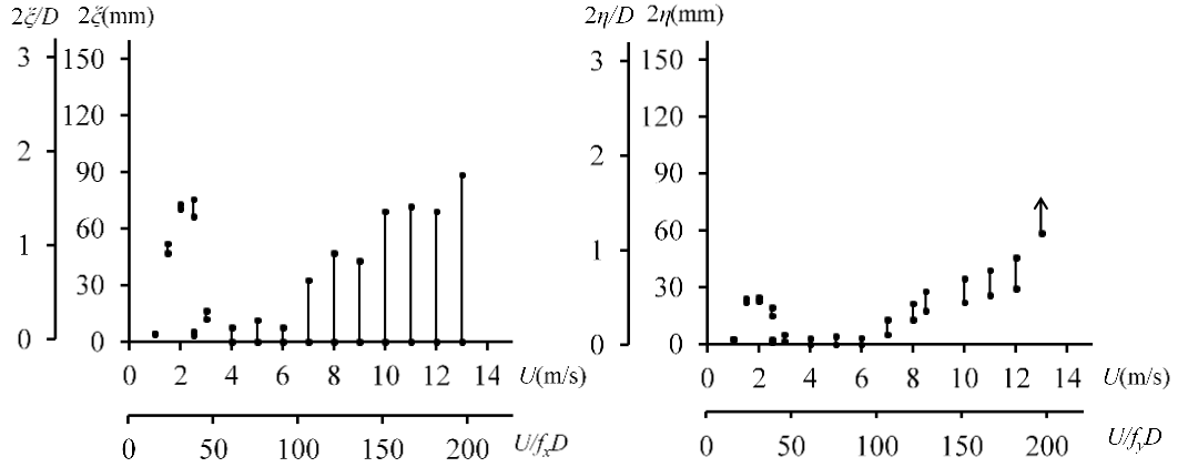
Fig. 15 Velocity–amplitude diagrams at ( X/D = 3.0 ; Y/D = 0.5 ) from the spring-supported free vibration test
