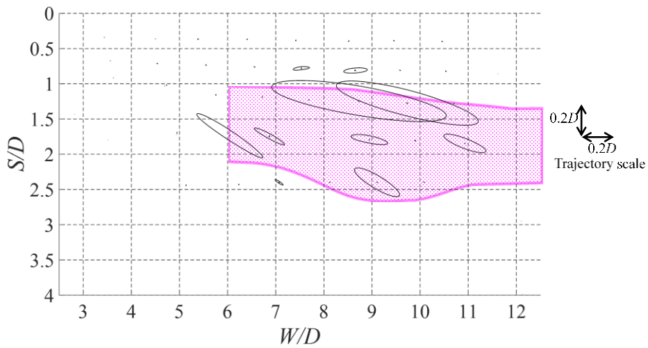
Fig. 13 Trajectories of the downstream cylinder calculated from the time-history analyses at U = 12 m/s ( U/fD = 177.8 )
