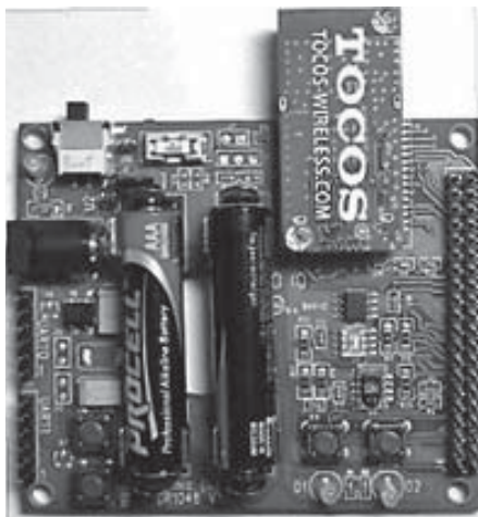
Figure 1. ZigBee device.
