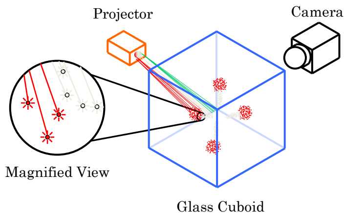
Fig. 1. The setup of the display with calibration system.
