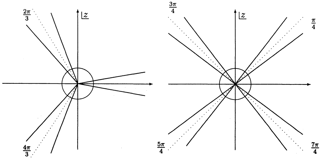
Figure 2: \Omega_\epsilon(0, 3, 1) and \Omega_\epsilon(0, 4, -1)
