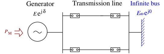
Figure 2 Single machine-infinite bus (SMIB) system
