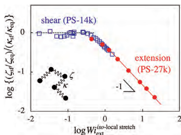
Figure 1. Comparison of the ratio of friction reduction factor \zeta_{sf}/\zeta_{eq} and spring strength reduction factor \kappa_{sf}/\kappa_{eq} against extensional Weissenberg number in the iso-local stretch condition Wi_{ext}^{iso-lu} for PS-14k under shear and PS-27k under extension.
