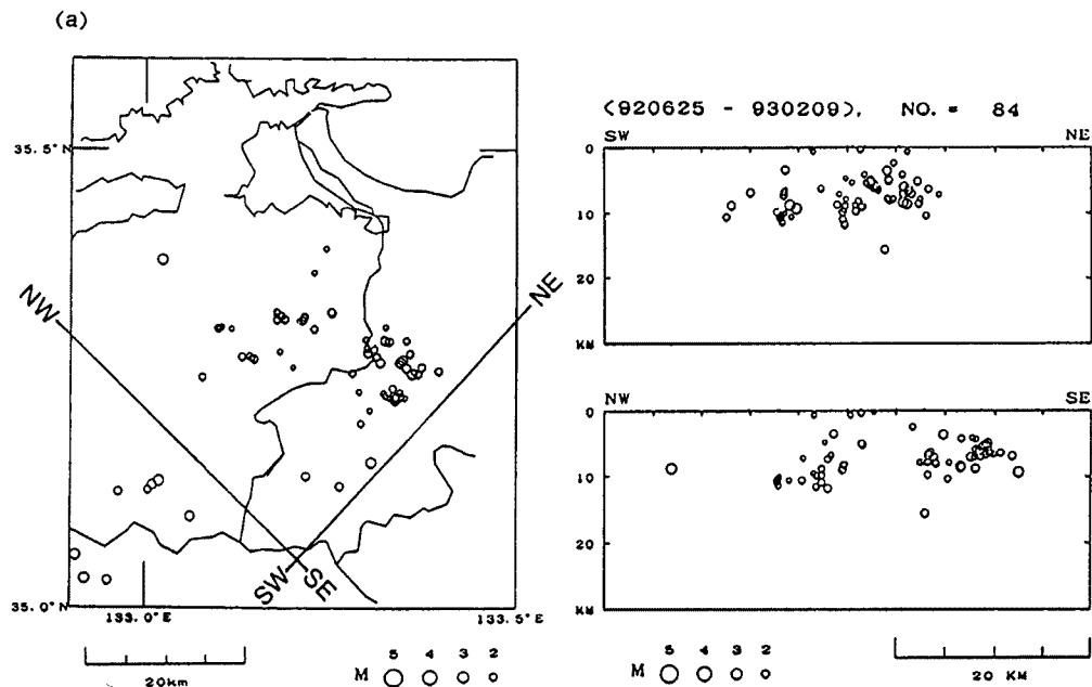
Fig. 9-(a). Seismic foci determined by temporary observation.
