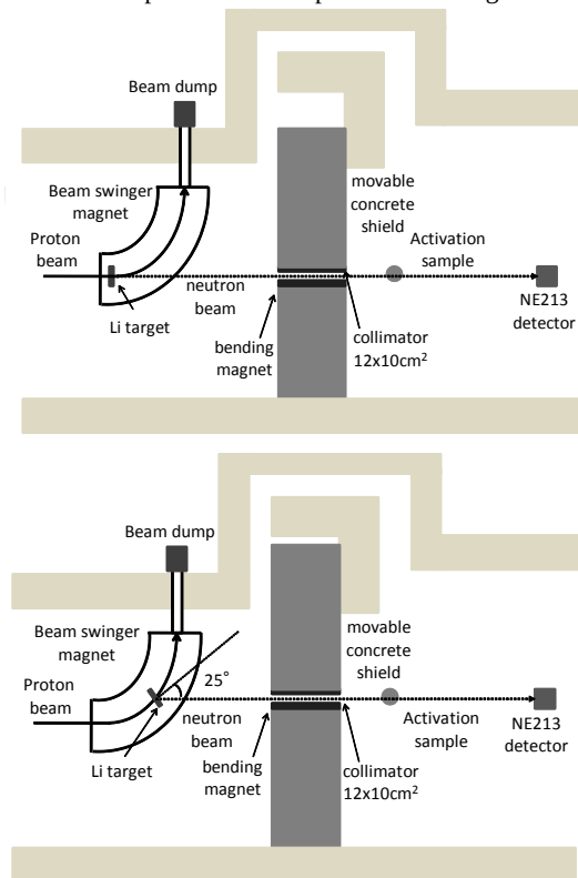
Figure 1. Schematic view of the experimental set up. (upper panel: 0° irradiation, lower panel: 25° irradiation)
