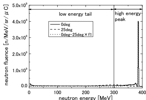
Figure 2. Neutron energy spectra generated by the ^7\text{Li}(p,n) reaction and corrected spectra obtained by subtracting the normalized 25° spectra from the 0° spectra.
