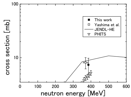
Figure 3(c). Excitation function for ^{209}\text{Bi}(n,x) ^{183g}\text{Os} reaction
