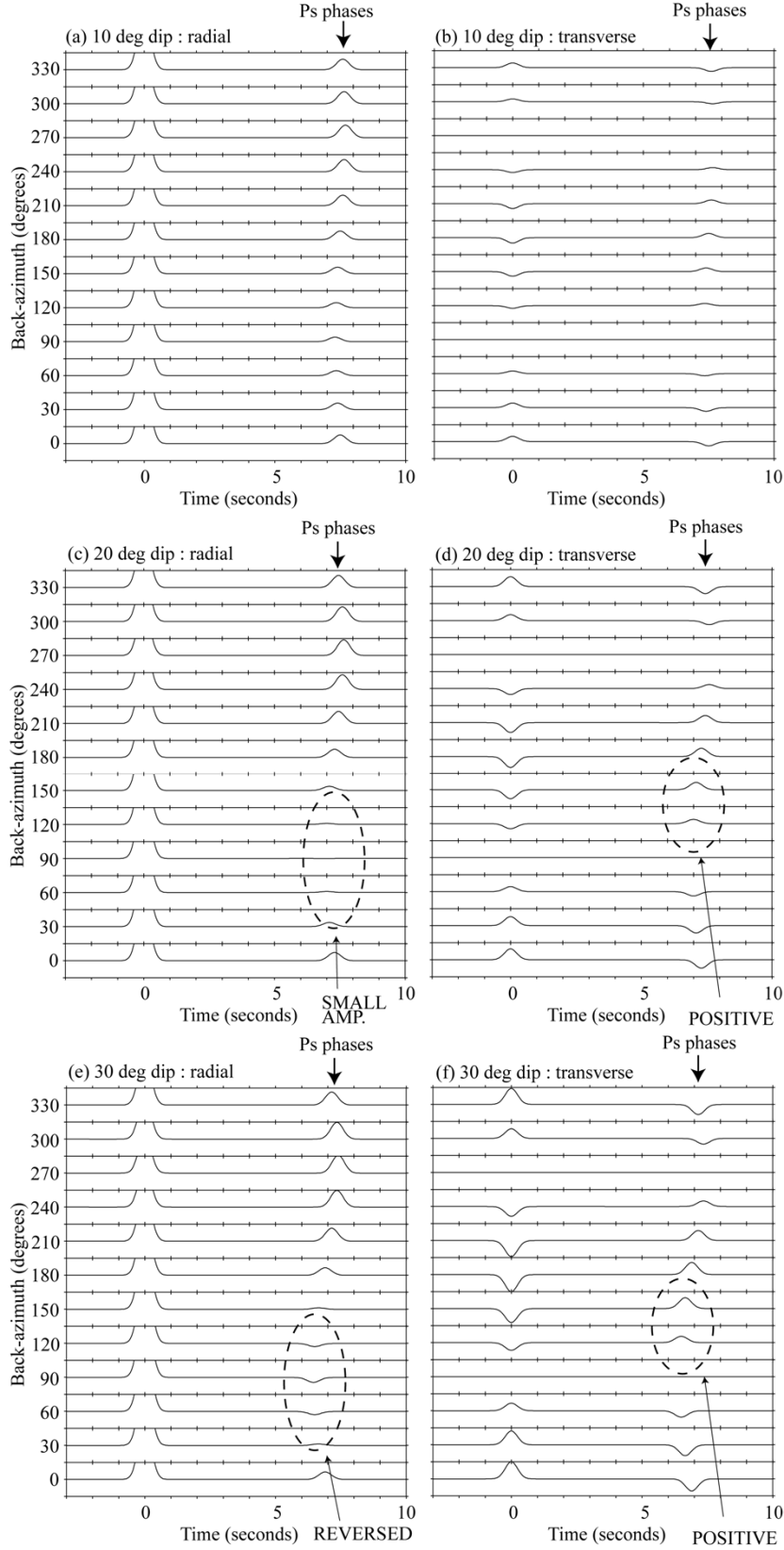
Figure 3 RFs synthesized with generalized ray theory assuming the two layered half space model. In each plate, RFs are shown in each 30° of back-azimuth. RF amplitudes from -0.1 to 0.1 are shown in order to make Ps converted phases more clear. (a,b) Radial and transverse RFs synthesized assuming the interface dips at 10°. (c,d) Those at 20°. (e,f) Those at 30°.
