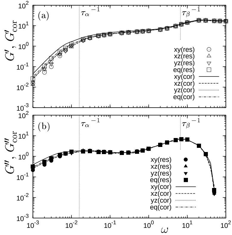
Figure 4.8: The response and correlation functions (a) G'_{\dot{\gamma}_s} and G'_{\text{cor}, \dot{\gamma}_s} and (b) G''_{\dot{\gamma}_s} and G''_{\text{cor}, \dot{\gamma}_s} versus \omega . \dot{\gamma}_s = 10^{-4} (weakly sheared state). We also show the functions in the equilibrium state. The symbols and lines represent the response functions and the correlation functions, respectively. The labels “res” and “cor” correspond to the response function and the correlation function, respectively. See also the caption of Fig. 4.3 for the labels “xy”, “xz”, “yz”, and “eq”.
