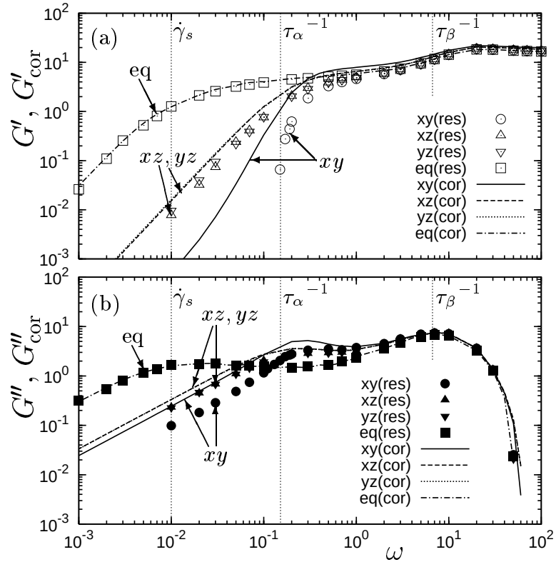
Figure 4.9: The response and correlation functions (a) G'_{\dot{\gamma}_s} and G'_{\text{cor}, \dot{\gamma}_s} and (b) G''_{\dot{\gamma}_s} and G''_{\text{cor}, \dot{\gamma}_s} versus \omega . \dot{\gamma}_s = 10^{-2} (strongly sheared state). See the caption of Fig. 4.8.
