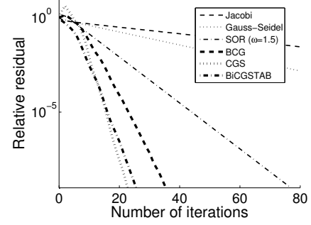
Fig. 1. Convergence of solution \mathbf{A}\mathbf{Q}^\mu = \bar{\mathbf{g}} , where \mathbf{A} is a general matrix.
