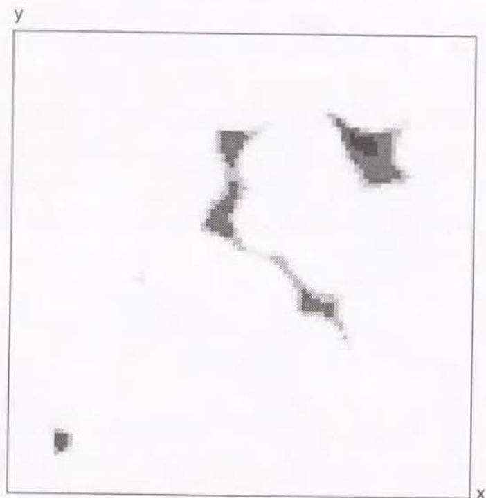
Figure 2.8. Energy map for a methane molecule in PDMS on an arbitrarily chosen plane parallel to the x - y plane. The energies are divided into five regions between U = -18, -8, 0 , and 10 kJ/mol; the lower energy region is painted darker.
