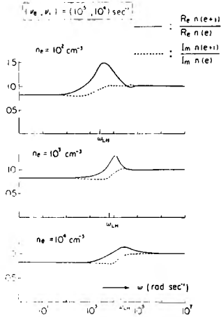
Fig. 5. Frequency dependence of a ratio of a refractive index with consideration for ions ( n(e+i) ) to that without ions ( n(e) ). The lower hybrid resonance frequency is shown by \omega_{LH} on the abscissa.
