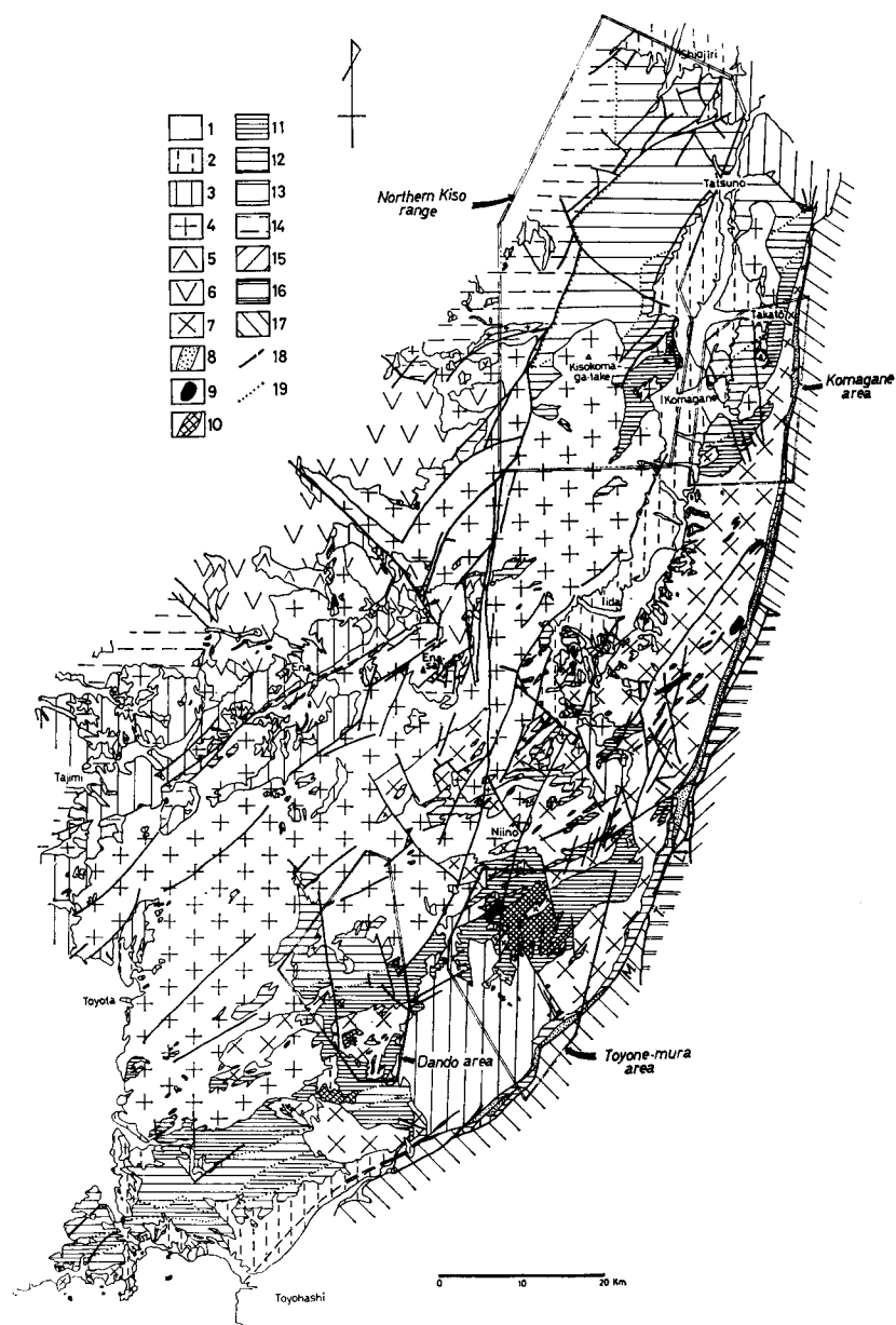
Fig. 1. Geological sketch-map of the Ryôke zone of central Japan, simplified from YAMADA et al. (1974).
