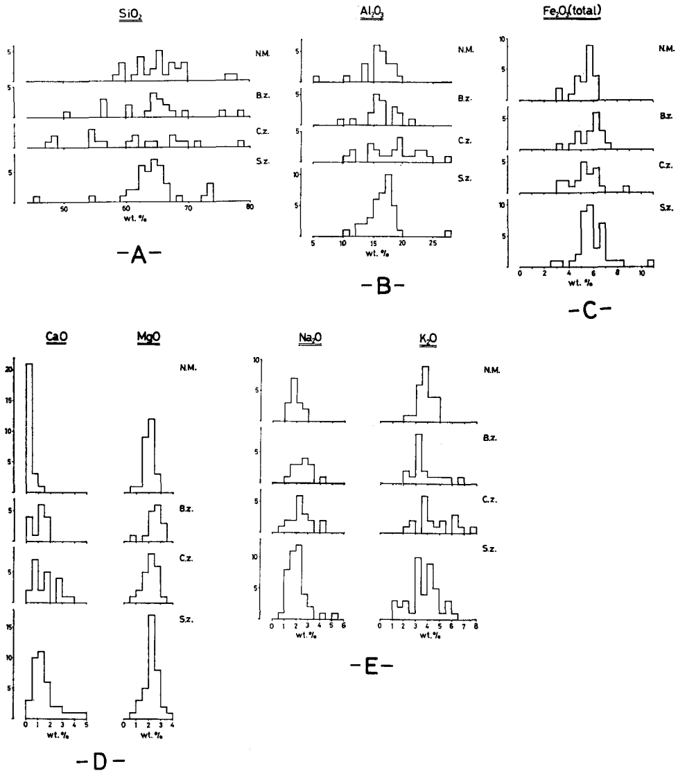
Fig. 3. Histograms for major element oxides of pelitic metamorphic and non-metamorphic rocks in zonal classification.
