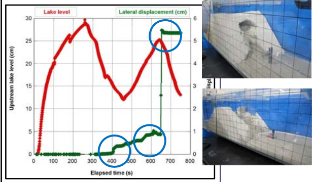
Plot of Upstream lake against Lateral displacement
