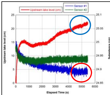
Plot of Upstream lake against Subsidence
