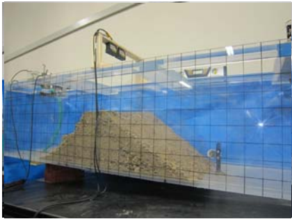
Akatani landslide dam model
